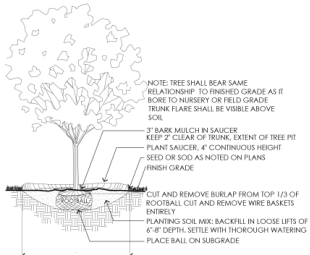
1 TYPICAL DECIDUOUS TREE PLANTING
