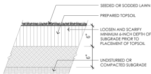
5 TYPICAL LAWN INSTALLATION
