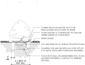
3 TYPICAL SHRUB PLANTING
