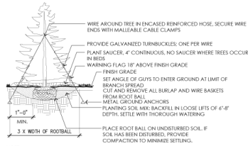
2 TYPICAL EVERGREEN TREE PLANTING
